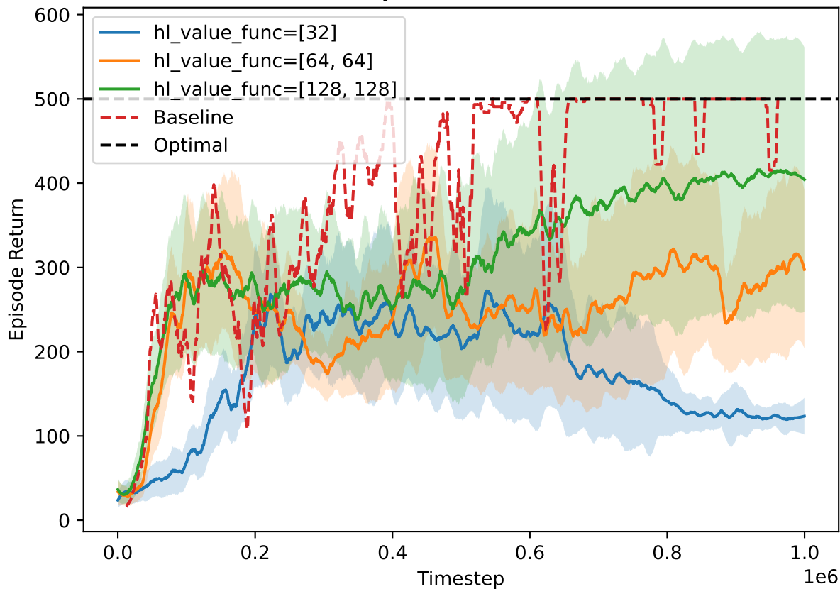
A2C hidden layers value function network
